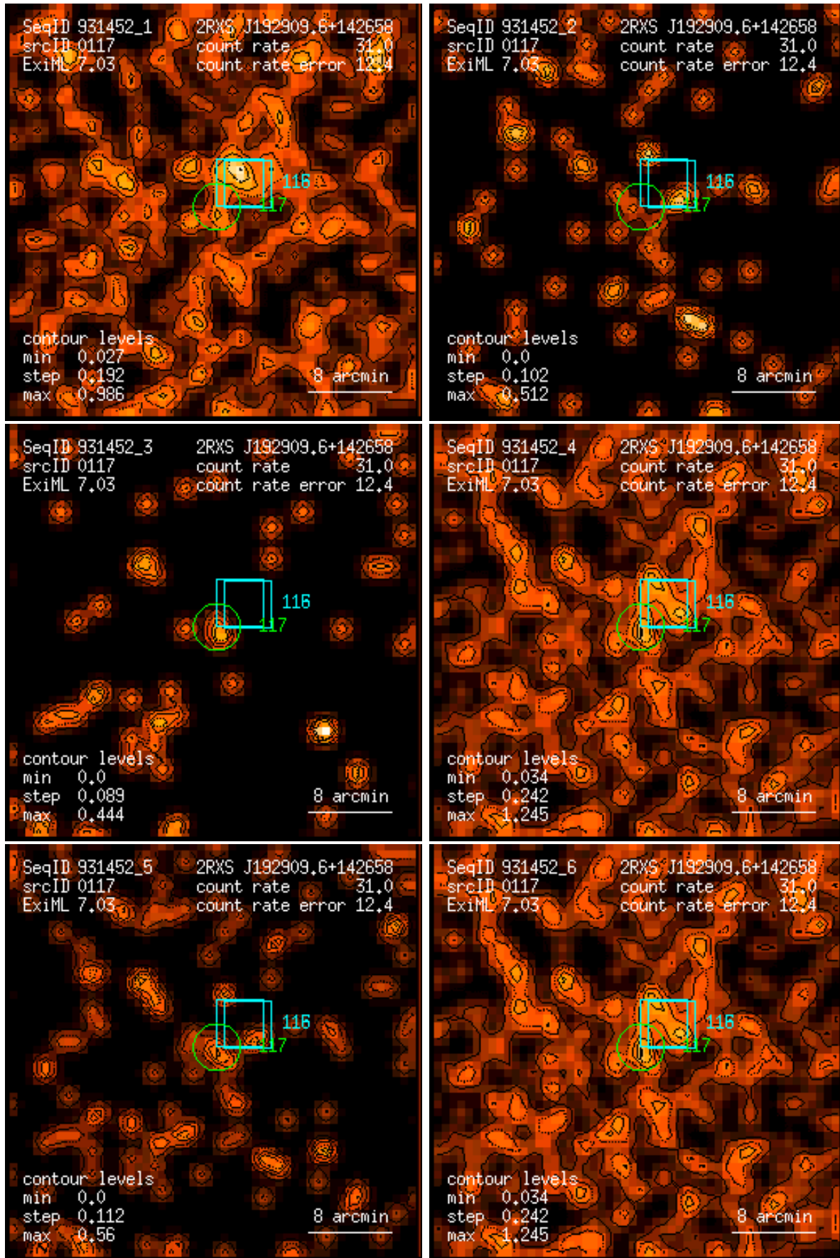
Figure 117: RASS 931452: detection 0117: band rate images, Gaussian filter: (1) PSPC channels 11 – 41, (2) 52 – 90, (3) 91 – 201, (4) 11 – 235, (5) 52 – 201, (6) 11 – 201. Broad band rates in counts/ks. Band rate contour levels in counts/ks/arcmin 2 .
