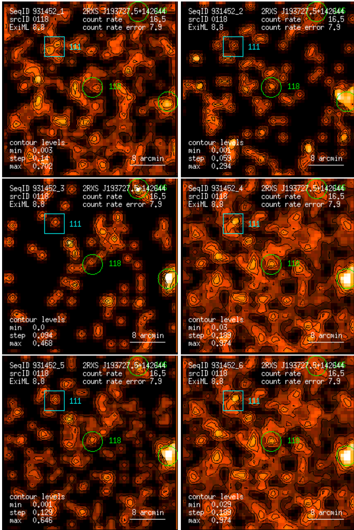
Figure 118: RASS 931452: detection 0118: band rate images, Gaussian filter: (1) PSPC channels 11 – 41, (2) 52 – 90, (3) 91 – 201, (4) 11 – 235, (5) 52 – 201, (6) 11 – 201. Broad band rates in counts/ks. Band rate contour levels in counts/ks/arcmin 2 .
