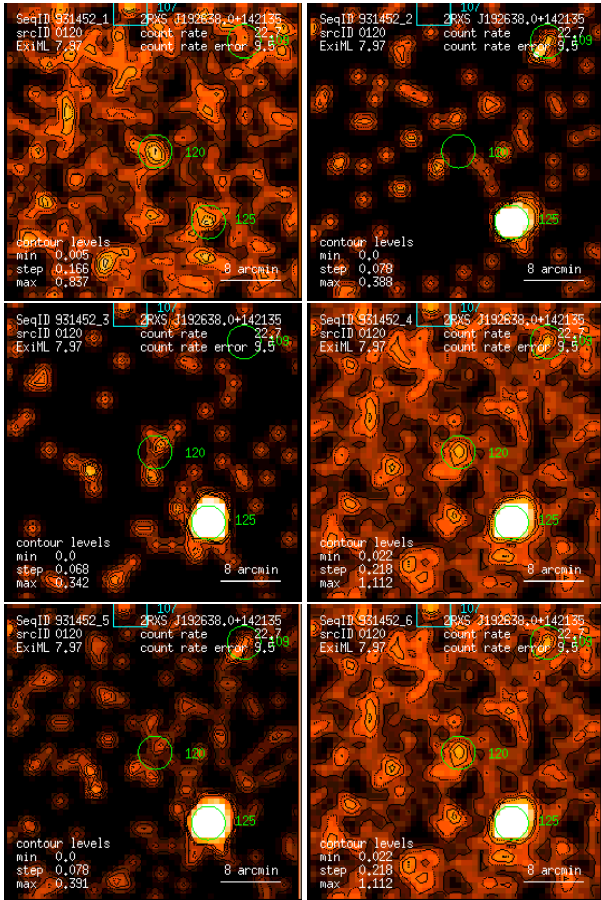
Figure 120: RASS 931452: detection 0120: band rate images, Gaussian filter: (1) PSPC channels 11 – 41, (2) 52 – 90, (3) 91 – 201, (4) 11 – 235, (5) 52 – 201, (6) 11 – 201. Broad band rates in counts/ks. Band rate contour levels in counts/ks/arcmin 2 .
