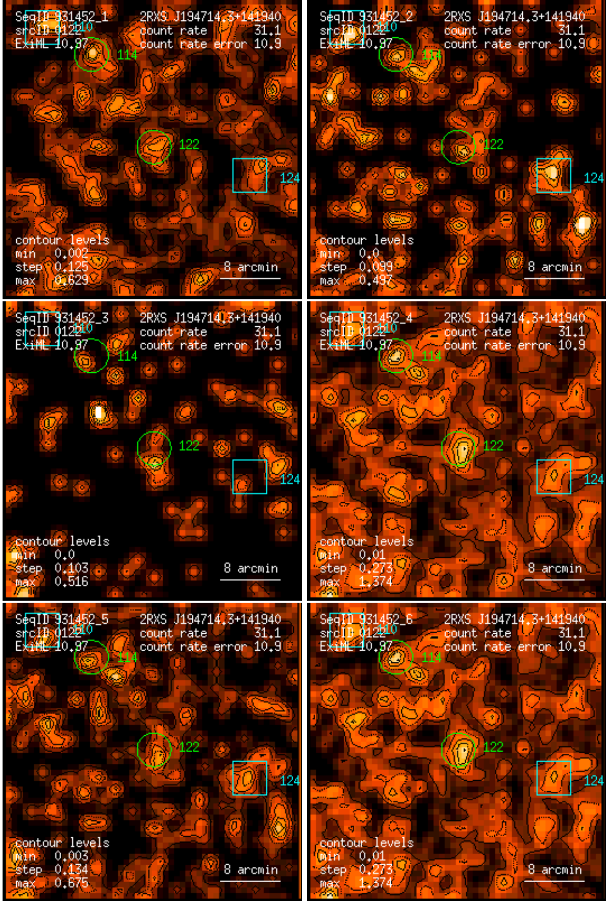
Figure 122: RASS 931452: detection 0122: band rate images, Gaussian filter: (1) PSPC channels 11 – 41, (2) 52 – 90, (3) 91 – 201, (4) 11 – 235, (5) 52 – 201, (6) 11 – 201. Broad band rates in counts/ks. Band rate contour levels in counts/ks/arcmin 2 .
