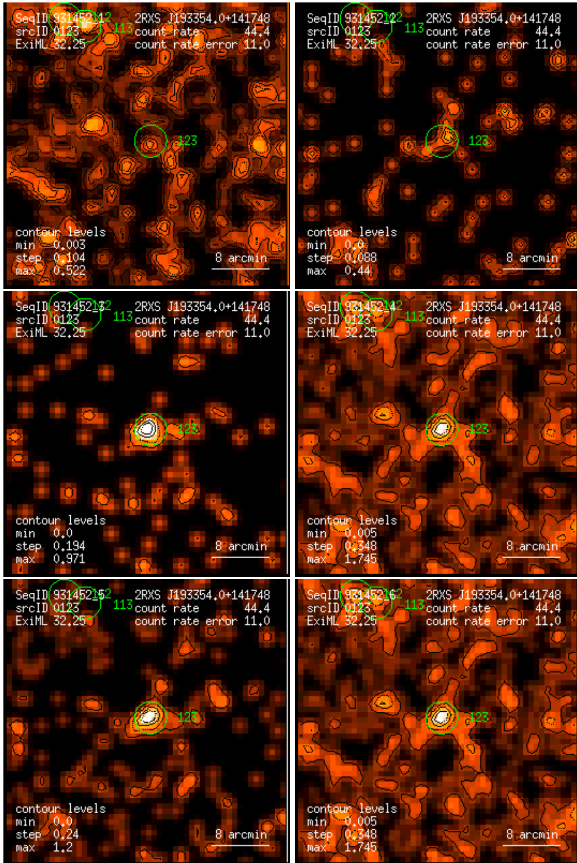
Figure 123: RASS 931452: detection 0123: band rate images, Gaussian filter: (1) PSPC channels 11 – 41, (2) 52 – 90, (3) 91 – 201, (4) 11 – 235, (5) 52 – 201, (6) 11 – 201. Broad band rates in counts/ks. Band rate contour levels in counts/ks/arcmin 2 .
