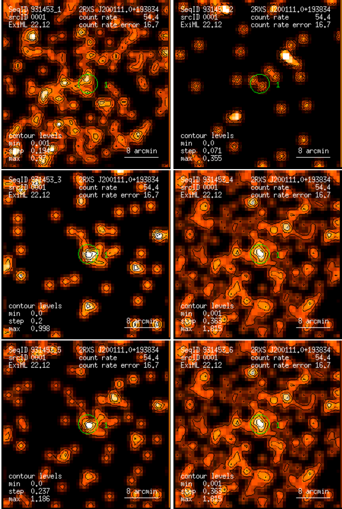
Figure 1: RASS 931453: detection 0001: band rate images, Gaussian filter: (1) PSPC channels 11 – 41, (2) 52 – 90, (3) 91 – 201, (4) 11 – 235, (5) 52 – 201, (6) 11 – 201. Broad band rates in counts/ks. Band rate contour levels in counts/ks/arcmin 2 .
