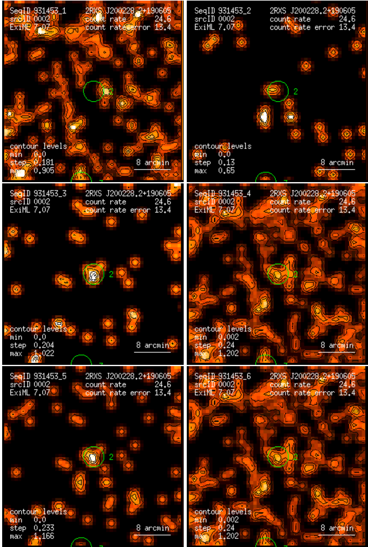
Figure 2: RASS 931453: detection 0002: band rate images, Gaussian filter: (1) PSPC channels 11 – 41, (2) 52 – 90, (3) 91 – 201, (4) 11 – 235, (5) 52 – 201, (6) 11 – 201. Broad band rates in counts/ks. Band rate contour levels in counts/ks/arcmin 2 .
