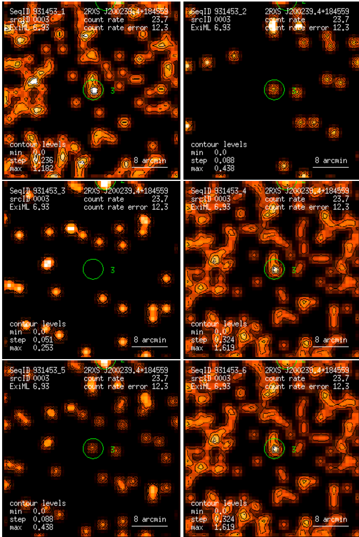
Figure 3: RASS 931453: detection 0003: band rate images, Gaussian filter: (1) PSPC channels 11 – 41, (2) 52 – 90, (3) 91 – 201, (4) 11 – 235, (5) 52 – 201, (6) 11 – 201. Broad band rates in counts/ks. Band rate contour levels in counts/ks/arcmin 2 .
