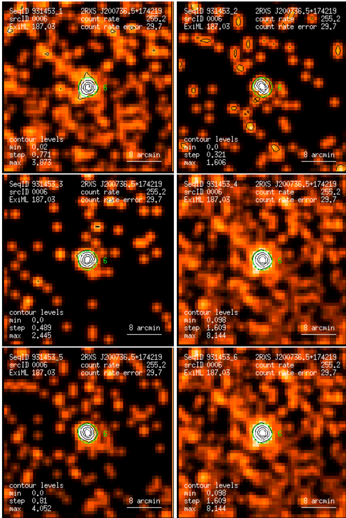
Figure 6: RASS 931453: detection 0006: band rate images, Gaussian filter: (1) PSPC channels 11 – 41, (2) 52 – 90, (3) 91 – 201, (4) 11 – 235, (5) 52 – 201, (6) 11 – 201. Broad band rates in counts/ks. Band rate contour levels in counts/ks/arcmin 2 .
