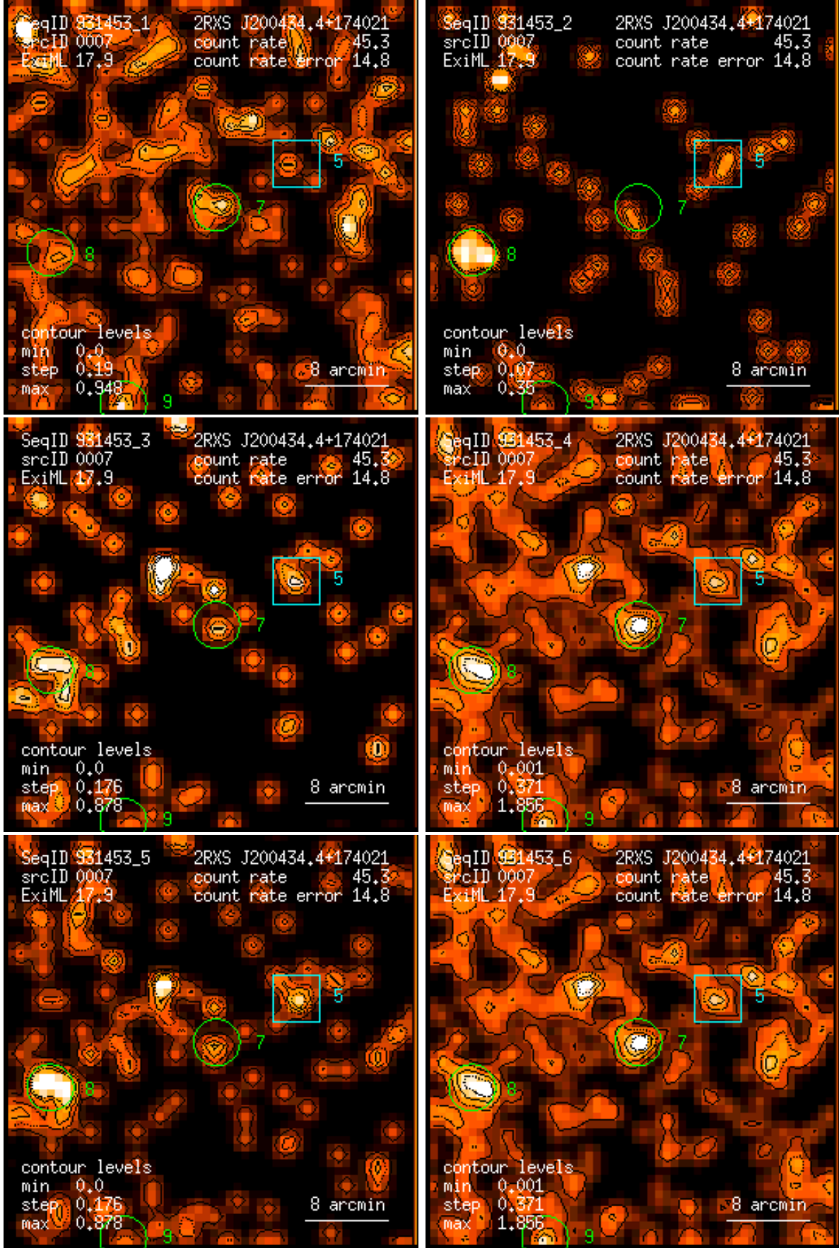
Figure 7: RASS 931453: detection 0007: band rate images, Gaussian filter: (1) PSPC channels 11 – 41, (2) 52 – 90, (3) 91 – 201, (4) 11 – 235, (5) 52 – 201, (6) 11 – 201. Broad band rates in counts/ks. Band rate contour levels in counts/ks/arcmin 2 .
