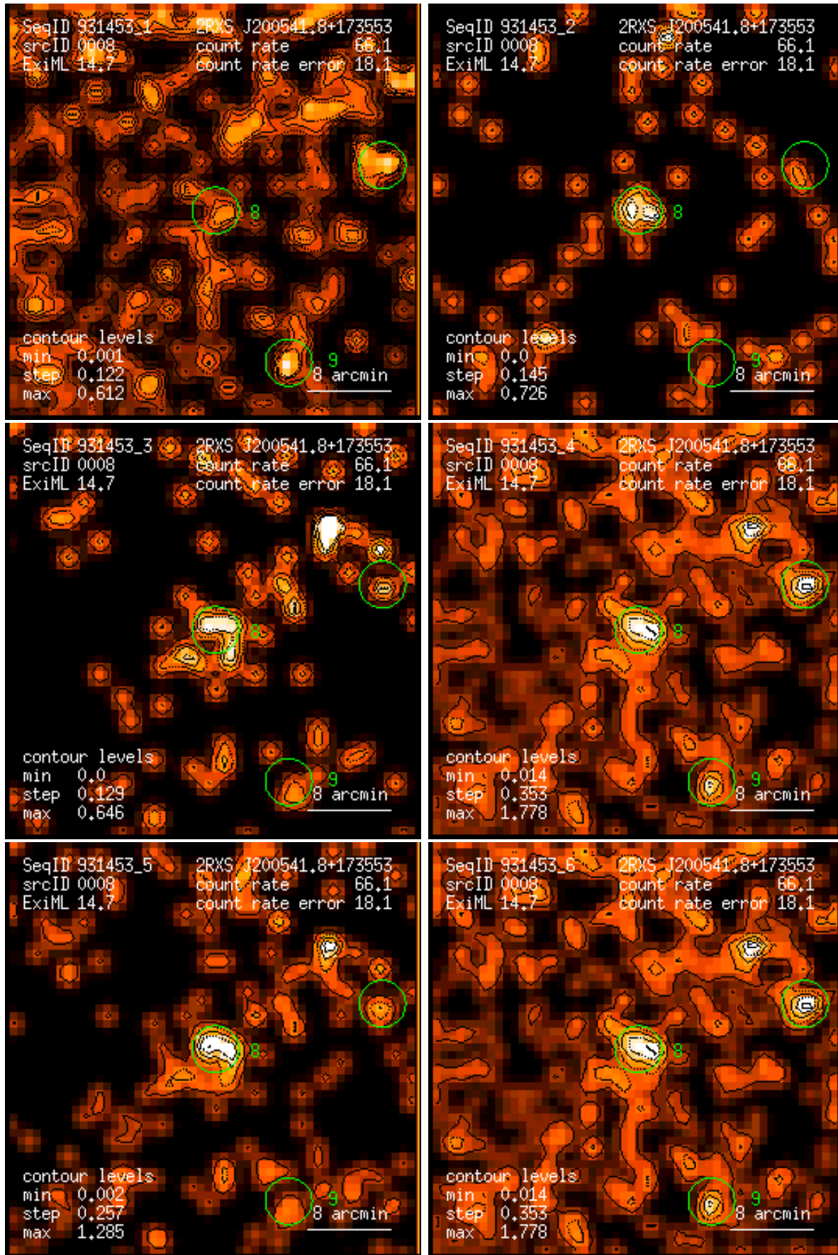
Figure 8: RASS 931453: detection 0008: band rate images, Gaussian filter: (1) PSPC channels 11 – 41, (2) 52 – 90, (3) 91 – 201, (4) 11 – 235, (5) 52 – 201, (6) 11 – 201. Broad band rates in counts/ks. Band rate contour levels in counts/ks/arcmin 2 .
