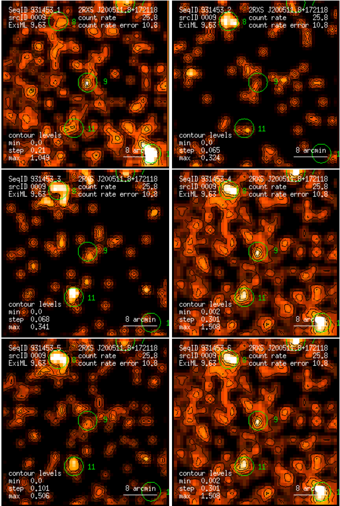
Figure 9: RASS 931453: detection 0009: band rate images, Gaussian filter: (1) PSPC channels 11 – 41, (2) 52 – 90, (3) 91 – 201, (4) 11 – 235, (5) 52 – 201, (6) 11 – 201. Broad band rates in counts/ks. Band rate contour levels in counts/ks/arcmin 2 .
