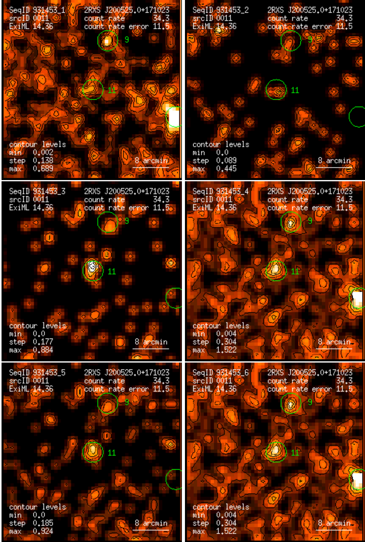
Figure 11: RASS 931453: detection 0011: band rate images, Gaussian filter: (1) PSPC channels 11 – 41, (2) 52 – 90, (3) 91 – 201, (4) 11 – 235, (5) 52 – 201, (6) 11 – 201. Broad band rates in counts/ks. Band rate contour levels in counts/ks/arcmin 2 .
