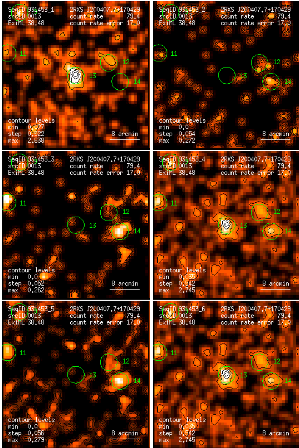
Figure 13: RASS 931453: detection 0013: band rate images, Gaussian filter: (1) PSPC channels 11 – 41, (2) 52 – 90, (3) 91 – 201, (4) 11 – 235, (5) 52 – 201, (6) 11 – 201. Broad band rates in counts/ks. Band rate contour levels in counts/ks/arcmin 2 .
