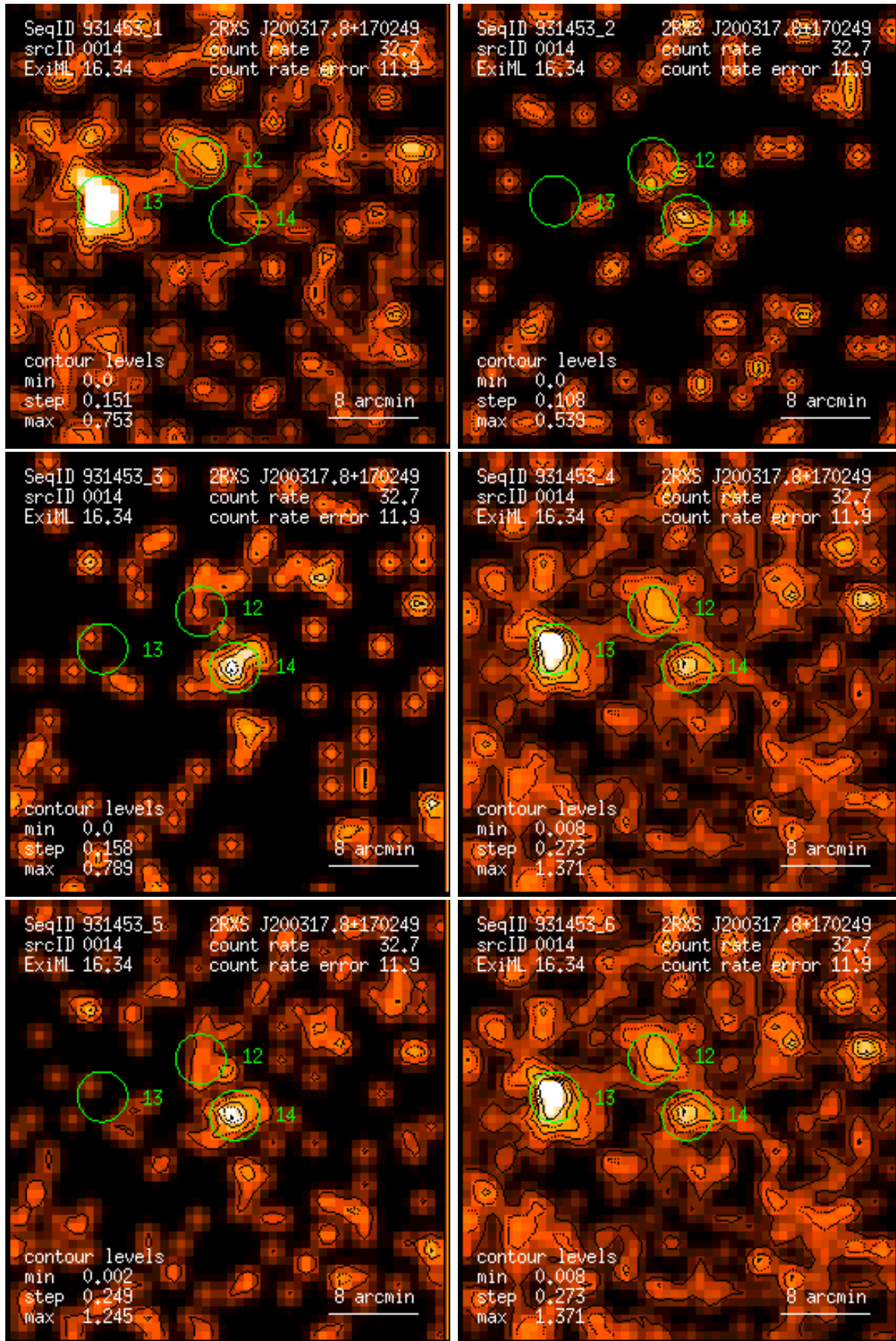
Figure 14: RASS 931453: detection 0014: band rate images, Gaussian filter: (1) PSPC channels 11 – 41, (2) 52 – 90, (3) 91 – 201, (4) 11 – 235, (5) 52 – 201, (6) 11 – 201. Broad band rates in counts/ks. Band rate contour levels in counts/ks/arcmin 2 .
