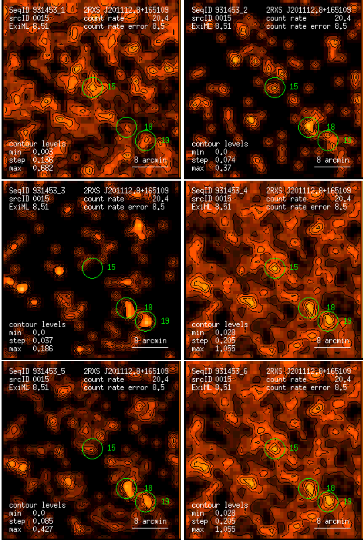
Figure 15: RASS 931453: detection 0015: band rate images, Gaussian filter: (1) PSPC channels 11 – 41, (2) 52 – 90, (3) 91 – 201, (4) 11 – 235, (5) 52 – 201, (6) 11 – 201. Broad band rates in counts/ks. Band rate contour levels in counts/ks/arcmin 2 .
