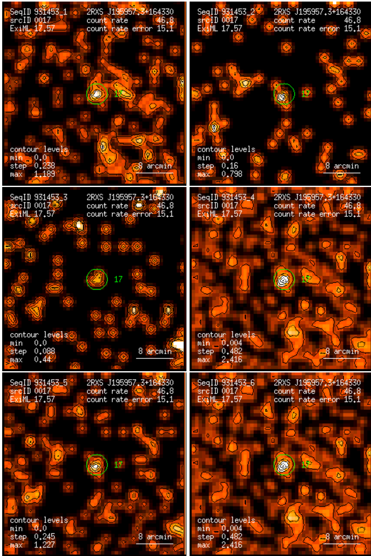
Figure 17: RASS 931453: detection 0017: band rate images, Gaussian filter: (1) PSPC channels 11 – 41, (2) 52 – 90, (3) 91 – 201, (4) 11 – 235, (5) 52 – 201, (6) 11 – 201. Broad band rates in counts/ks. Band rate contour levels in counts/ks/arcmin 2 .
