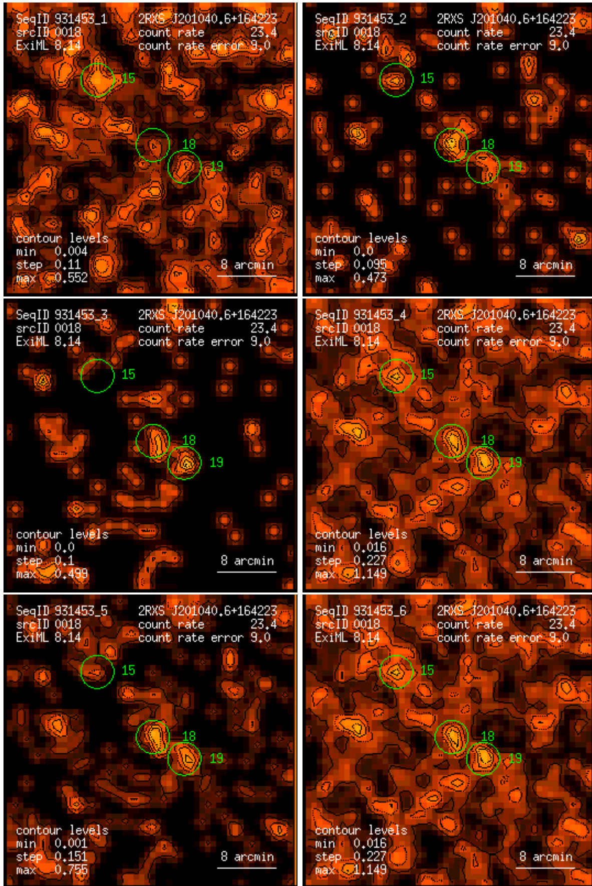
Figure 18: RASS 931453: detection 0018: band rate images, Gaussian filter: (1) PSPC channels 11 – 41, (2) 52 – 90, (3) 91 – 201, (4) 11 – 235, (5) 52 – 201, (6) 11 – 201. Broad band rates in counts/ks. Band rate contour levels in counts/ks/arcmin 2 .
