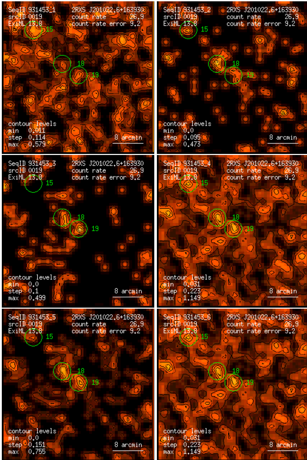
Figure 19: RASS 931453: detection 0019: band rate images, Gaussian filter: (1) PSPC channels 11 – 41, (2) 52 – 90, (3) 91 – 201, (4) 11 – 235, (5) 52 – 201, (6) 11 – 201. Broad band rates in counts/ks. Band rate contour levels in counts/ks/arcmin 2 .
