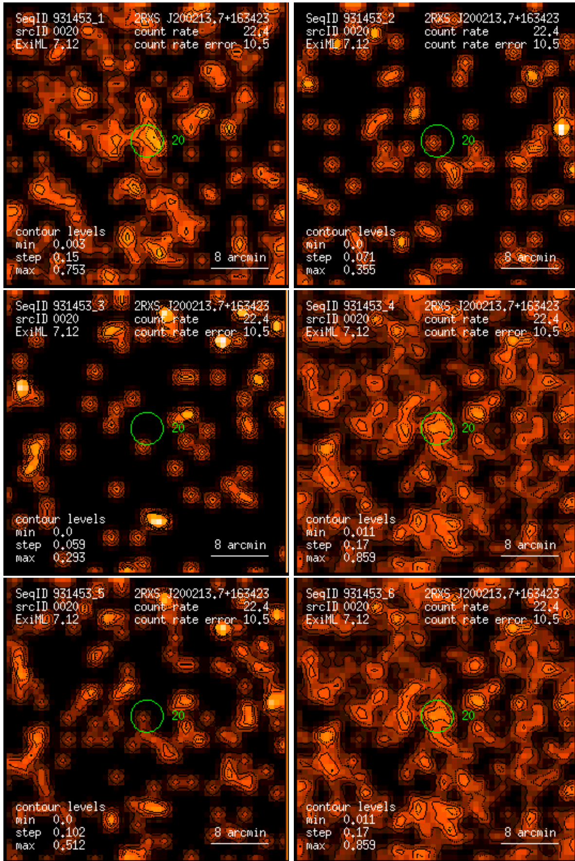
Figure 20: RASS 931453: detection 0020: band rate images, Gaussian filter: (1) PSPC channels 11 – 41, (2) 52 – 90, (3) 91 – 201, (4) 11 – 235, (5) 52 – 201, (6) 11 – 201. Broad band rates in counts/ks. Band rate contour levels in counts/ks/arcmin 2 .
