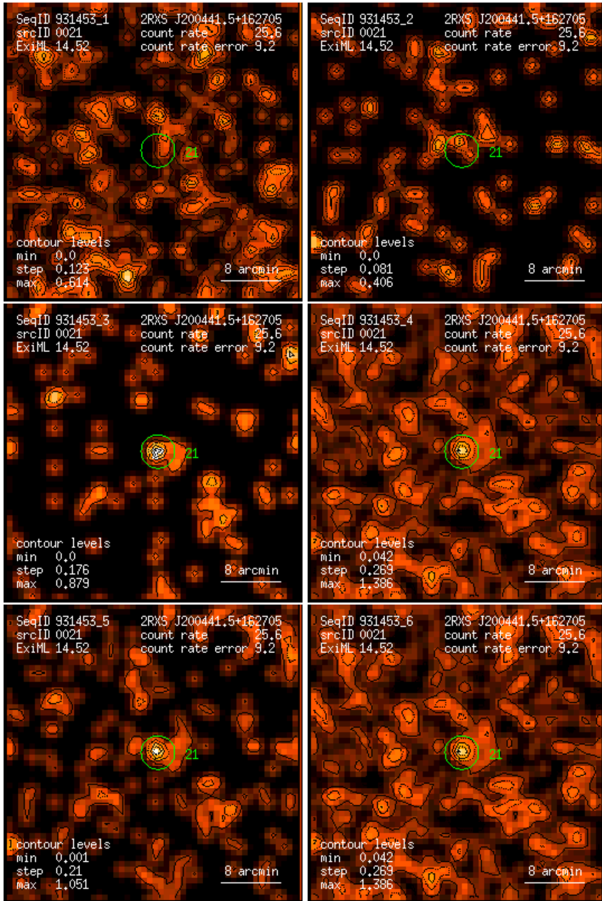
Figure 21: RASS 931453: detection 0021: band rate images, Gaussian filter: (1) PSPC channels 11 – 41, (2) 52 – 90, (3) 91 – 201, (4) 11 – 235, (5) 52 – 201, (6) 11 – 201. Broad band rates in counts/ks. Band rate contour levels in counts/ks/arcmin 2 .
