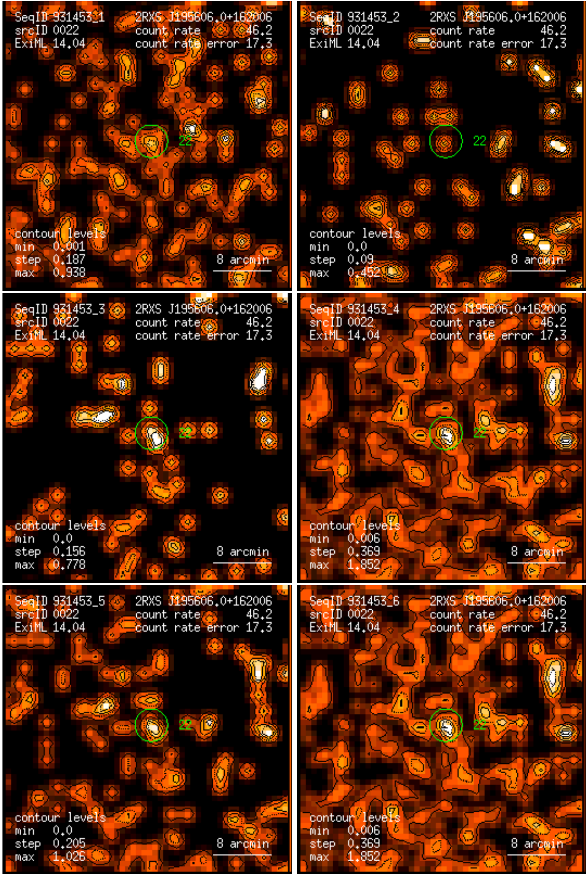
Figure 22: RASS 931453: detection 0022: band rate images, Gaussian filter: (1) PSPC channels 11 – 41, (2) 52 – 90, (3) 91 – 201, (4) 11 – 235, (5) 52 – 201, (6) 11 – 201. Broad band rates in counts/ks. Band rate contour levels in counts/ks/arcmin 2 .
