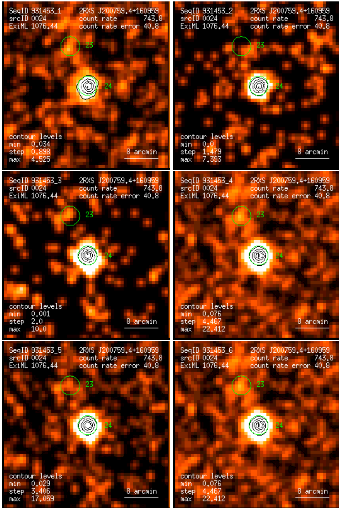
Figure 24: RASS 931453: detection 0024: band rate images, Gaussian filter: (1) PSPC channels 11 – 41, (2) 52 – 90, (3) 91 – 201, (4) 11 – 235, (5) 52 – 201, (6) 11 – 201. Broad band rates in counts/ks. Band rate contour levels in counts/ks/arcmin 2 .
