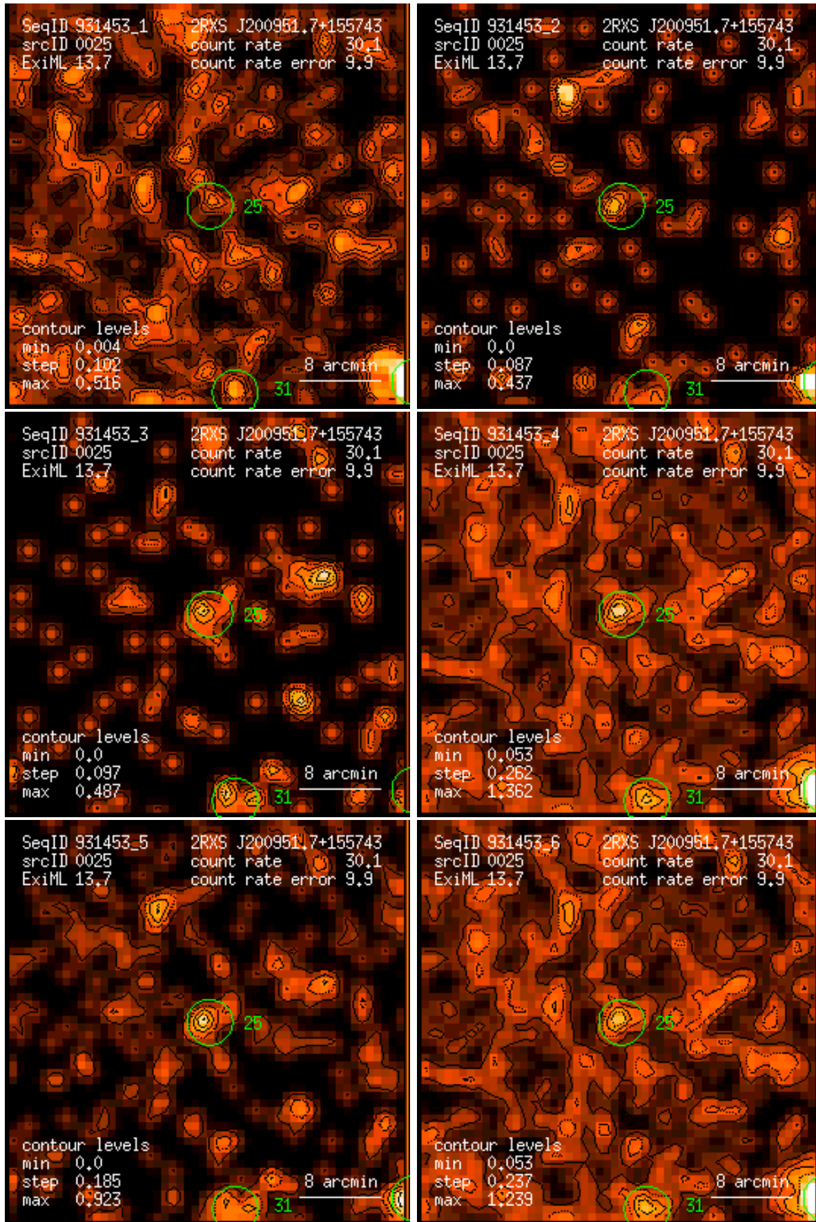
Figure 25: RASS 931453: detection 0025: band rate images, Gaussian filter: (1) PSPC channels 11 – 41, (2) 52 – 90, (3) 91 – 201, (4) 11 – 235, (5) 52 – 201, (6) 11 – 201. Broad band rates in counts/ks. Band rate contour levels in counts/ks/arcmin 2 .
