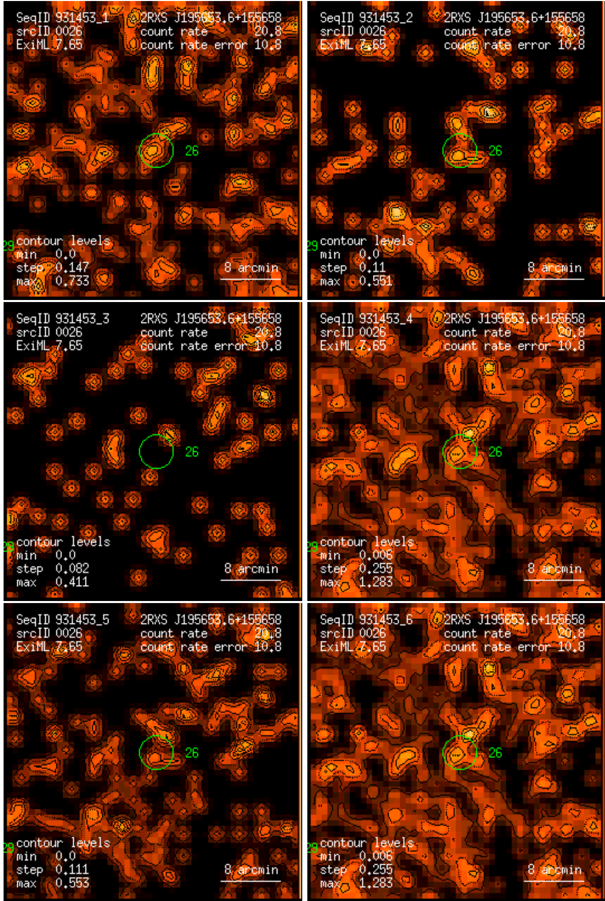
Figure 26: RASS 931453: detection 0026: band rate images, Gaussian filter: (1) PSPC channels 11 – 41, (2) 52 – 90, (3) 91 – 201, (4) 11 – 235, (5) 52 – 201, (6) 11 – 201. Broad band rates in counts/ks. Band rate contour levels in counts/ks/arcmin 2 .
