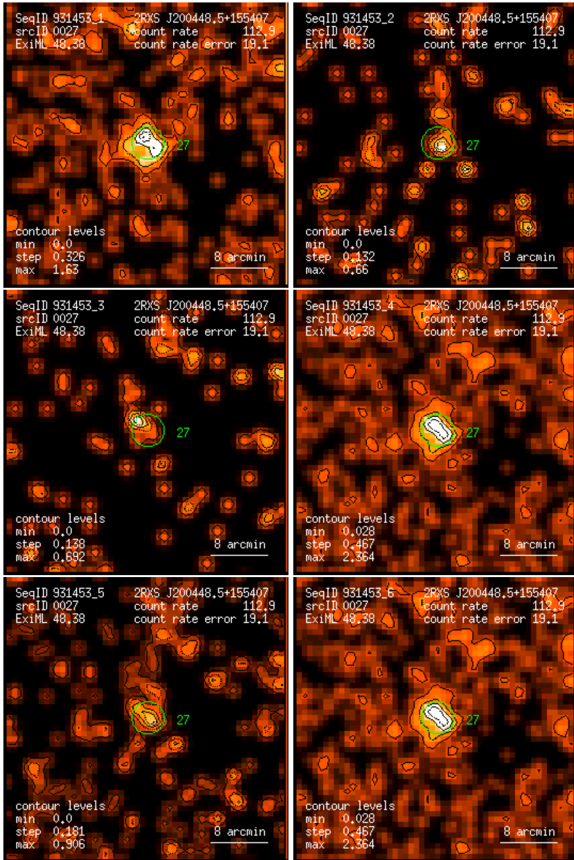
Figure 27: RASS 931453: detection 0027: band rate images, Gaussian filter: (1) PSPC channels 11 – 41, (2) 52 – 90, (3) 91 – 201, (4) 11 – 235, (5) 52 – 201, (6) 11 – 201. Broad band rates in counts/ks. Band rate contour levels in counts/ks/arcmin 2 .
