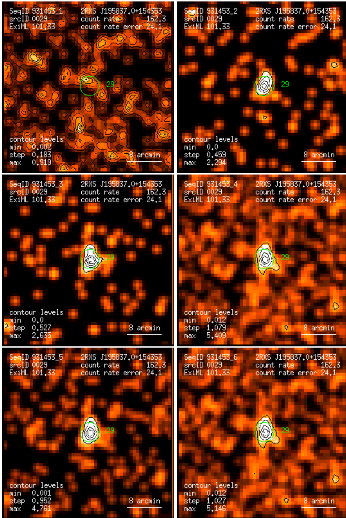
Figure 29: RASS 931453: detection 0029: band rate images, Gaussian filter: (1) PSPC channels 11 – 41, (2) 52 – 90, (3) 91 – 201, (4) 11 – 235, (5) 52 – 201, (6) 11 – 201. Broad band rates in counts/ks. Band rate contour levels in counts/ks/arcmin 2 .
