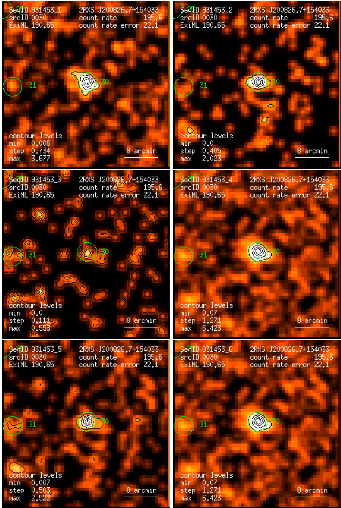
Figure 30: RASS 931453: detection 0030: band rate images, Gaussian filter: (1) PSPC channels 11 – 41, (2) 52 – 90, (3) 91 – 201, (4) 11 – 235, (5) 52 – 201, (6) 11 – 201. Broad band rates in counts/ks. Band rate contour levels in counts/ks/arcmin 2 .
