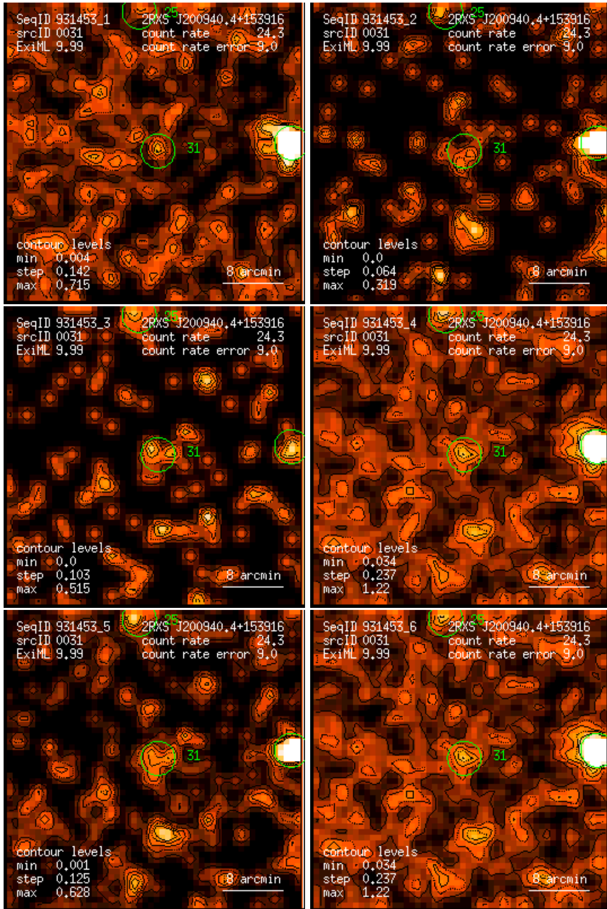
Figure 31: RASS 931453: detection 0031: band rate images, Gaussian filter: (1) PSPC channels 11 – 41, (2) 52 – 90, (3) 91 – 201, (4) 11 – 235, (5) 52 – 201, (6) 11 – 201. Broad band rates in counts/ks. Band rate contour levels in counts/ks/arcmin 2 .
