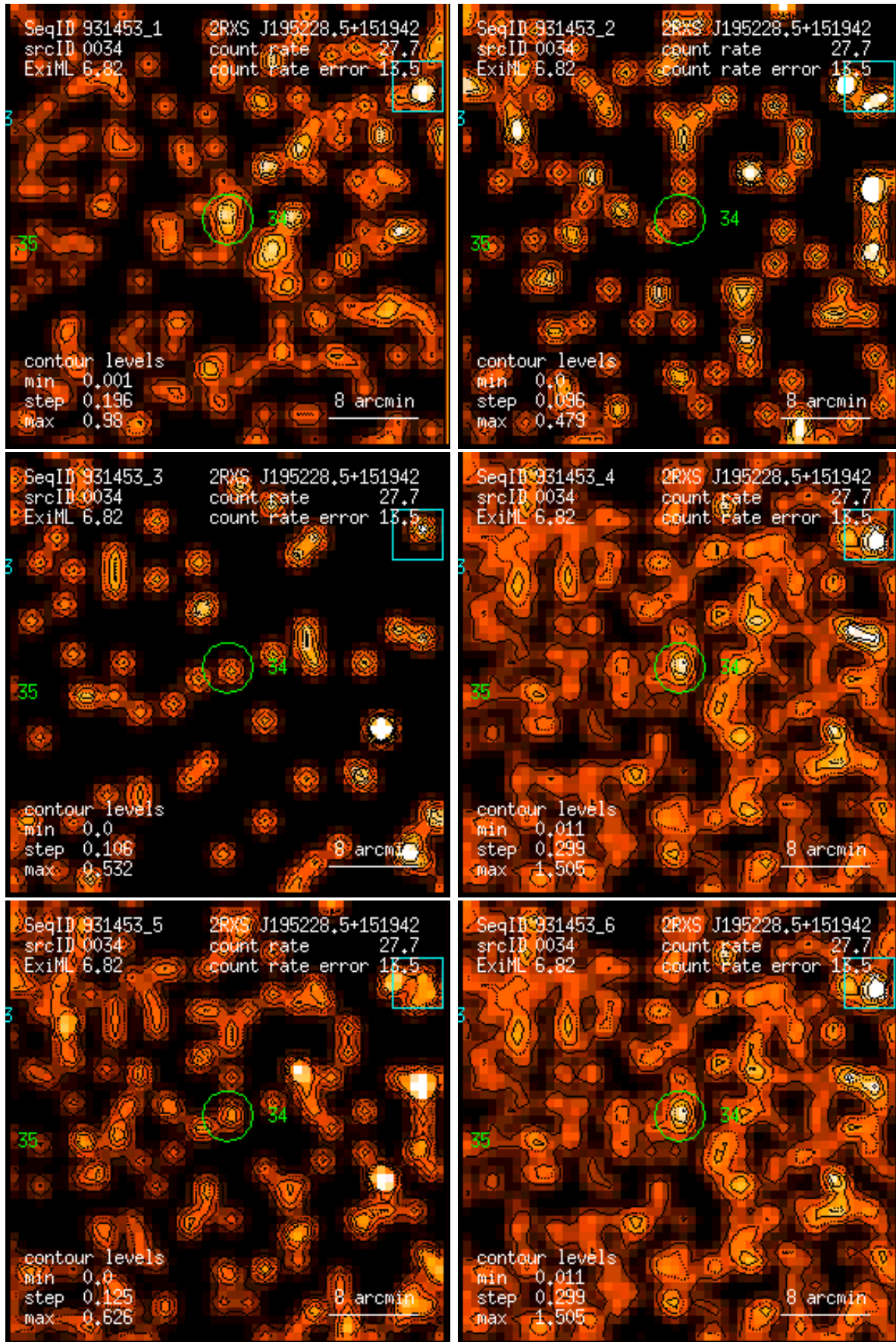
Figure 34: RASS 931453: detection 0034: band rate images, Gaussian filter: (1) PSPC channels 11 – 41, (2) 52 – 90, (3) 91 – 201, (4) 11 – 235, (5) 52 – 201, (6) 11 – 201. Broad band rates in counts/ks. Band rate contour levels in counts/ks/arcmin 2 .
