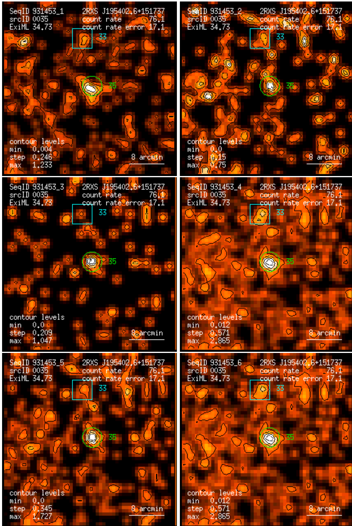
Figure 35: RASS 931453: detection 0035: band rate images, Gaussian filter: (1) PSPC channels 11 – 41, (2) 52 – 90, (3) 91 – 201, (4) 11 – 235, (5) 52 – 201, (6) 11 – 201. Broad band rates in counts/ks. Band rate contour levels in counts/ks/arcmin 2 .
