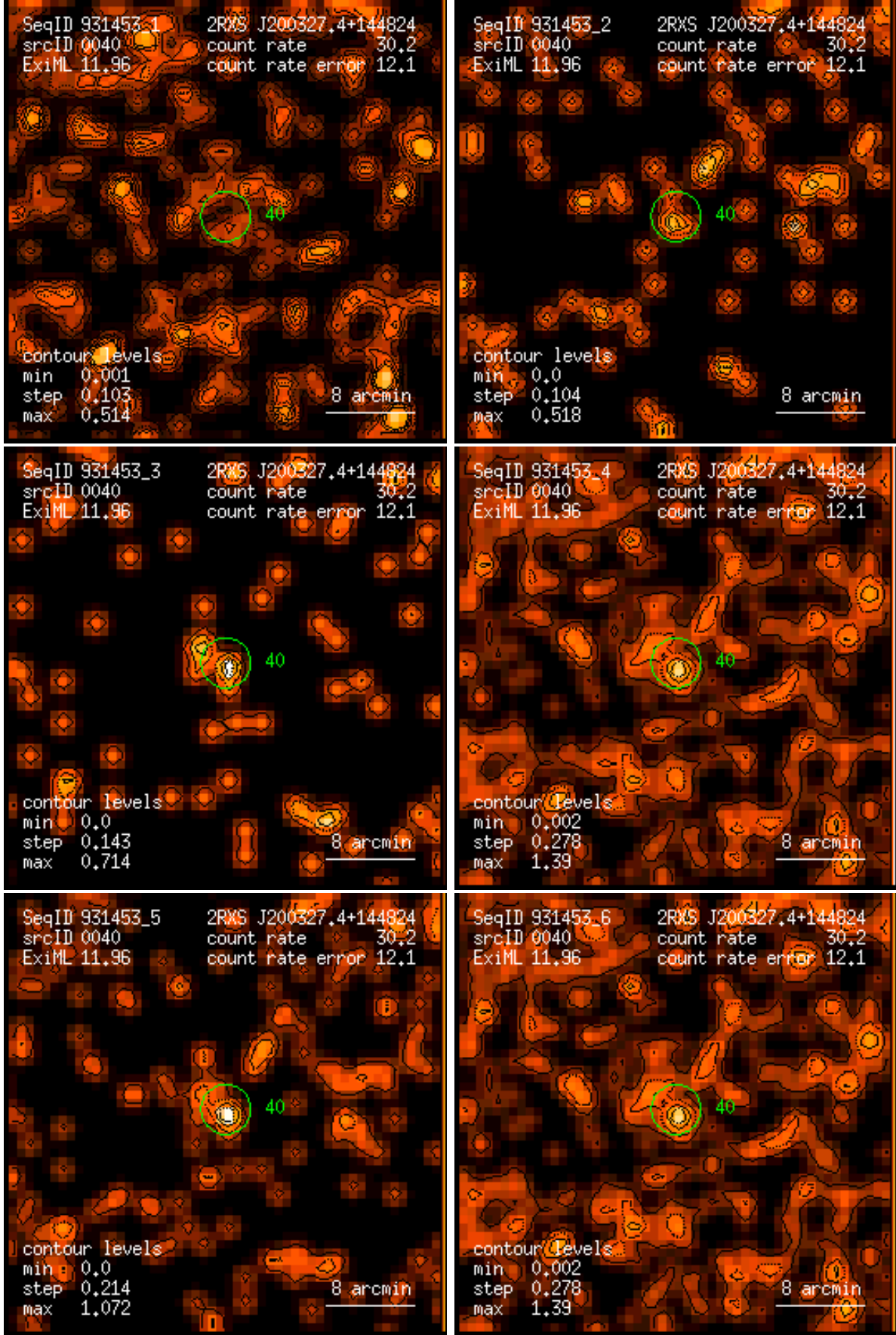
Figure 40: RASS 931453: detection 0040: band rate images, Gaussian filter: (1) PSPC channels 11 – 41, (2) 52 – 90, (3) 91 – 201, (4) 11 – 235, (5) 52 – 201, (6) 11 – 201. Broad band rates in counts/ks. Band rate contour levels in counts/ks/arcmin 2 .
