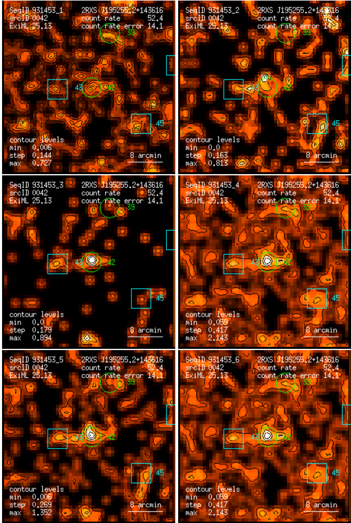
Figure 42: RASS 931453: detection 0042: band rate images, Gaussian filter: (1) PSPC channels 11 – 41, (2) 52 – 90, (3) 91 – 201, (4) 11 – 235, (5) 52 – 201, (6) 11 – 201. Broad band rates in counts/ks. Band rate contour levels in counts/ks/arcmin 2 .
