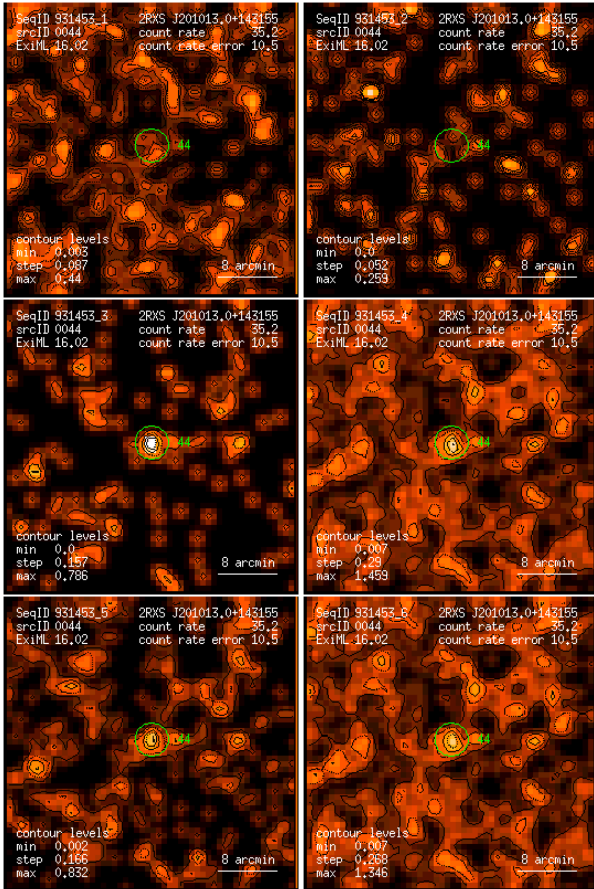
Figure 44: RASS 931453: detection 0044: band rate images, Gaussian filter: (1) PSPC channels 11 – 41, (2) 52 – 90, (3) 91 – 201, (4) 11 – 235, (5) 52 – 201, (6) 11 – 201. Broad band rates in counts/ks. Band rate contour levels in counts/ks/arcmin 2 .
