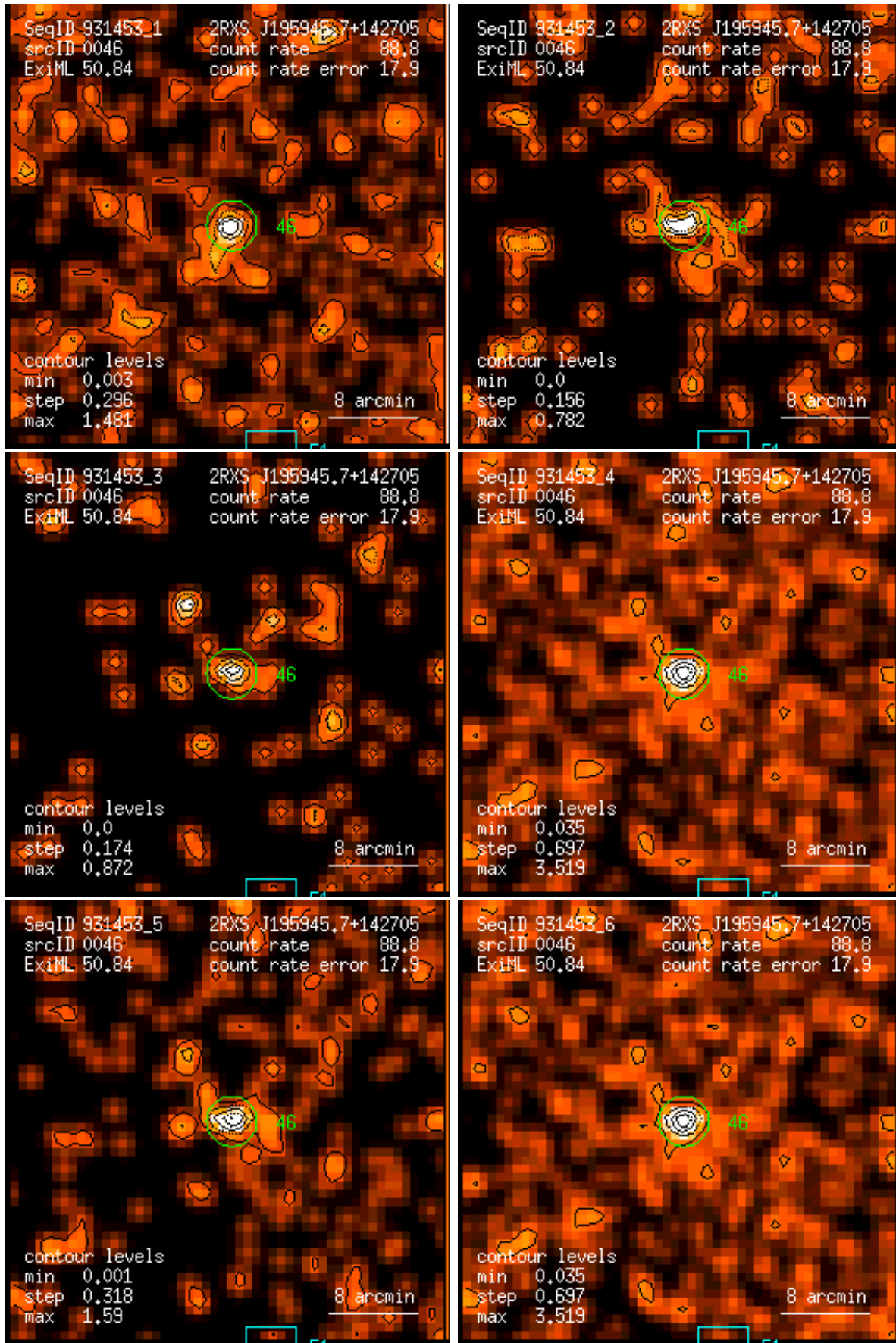
Figure 46: RASS 931453: detection 0046: band rate images, Gaussian filter: (1) PSPC channels 11 – 41, (2) 52 – 90, (3) 91 – 201, (4) 11 – 235, (5) 52 – 201, (6) 11 – 201. Broad band rates in counts/ks. Band rate contour levels in counts/ks/arcmin 2 .
