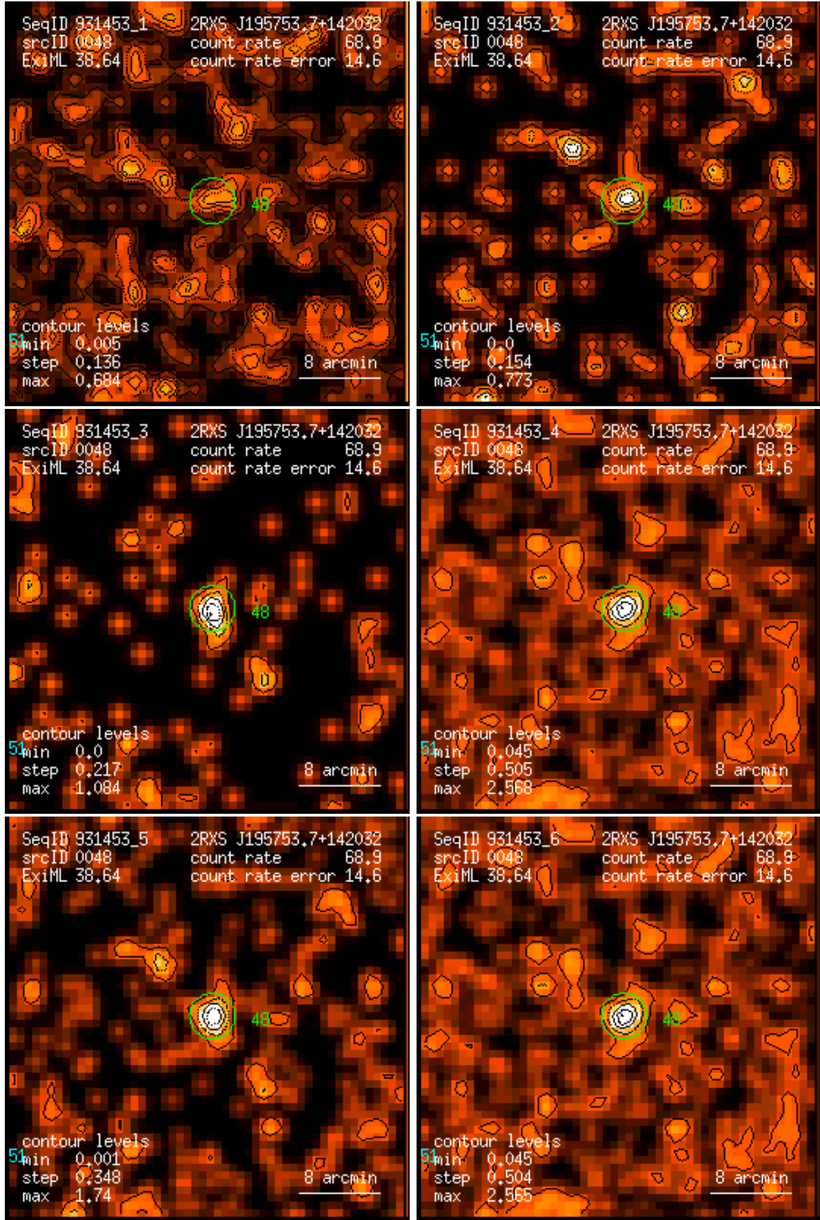
Figure 48: RASS 931453: detection 0048: band rate images, Gaussian filter: (1) PSPC channels 11 – 41, (2) 52 – 90, (3) 91 – 201, (4) 11 – 235, (5) 52 – 201, (6) 11 – 201. Broad band rates in counts/ks. Band rate contour levels in counts/ks/arcmin 2 .
