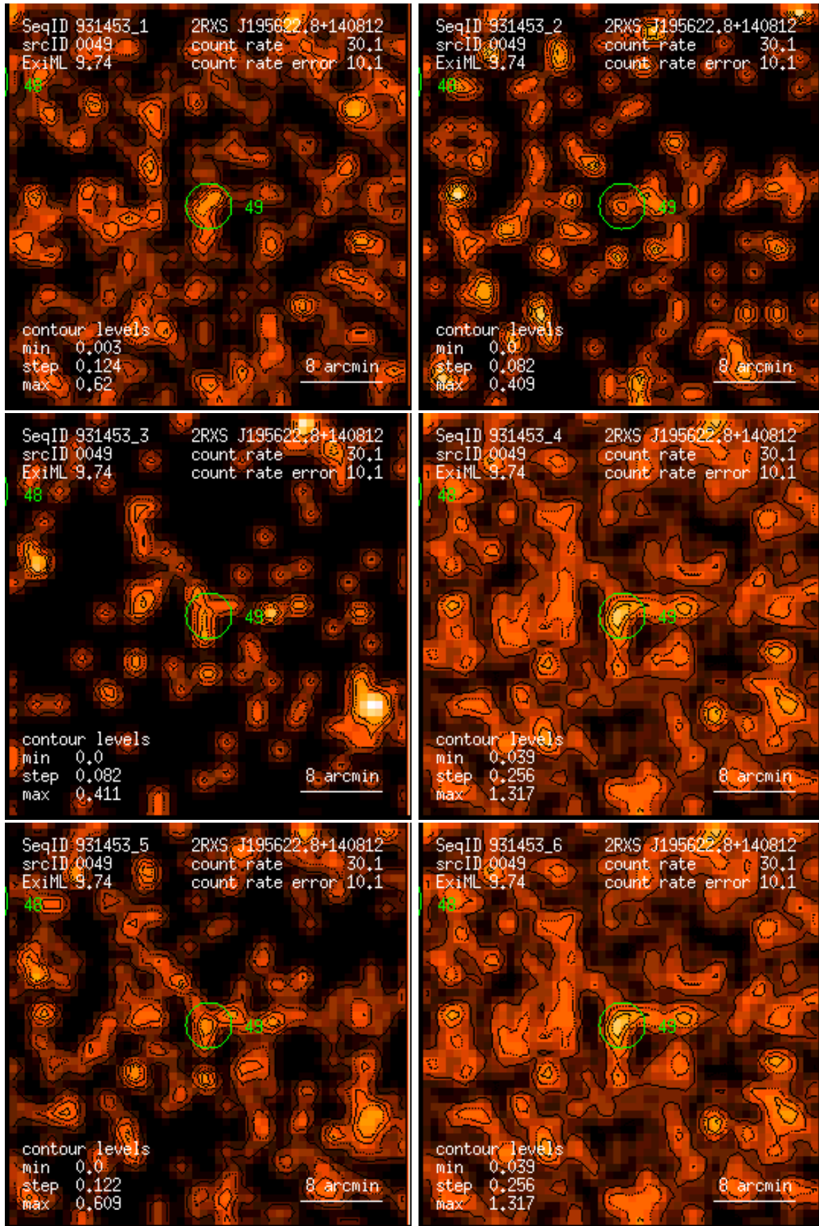
Figure 49: RASS 931453: detection 0049: band rate images, Gaussian filter: (1) PSPC channels 11 – 41, (2) 52 – 90, (3) 91 – 201, (4) 11 – 235, (5) 52 – 201, (6) 11 – 201. Broad band rates in counts/ks. Band rate contour levels in counts/ks/arcmin 2 .
