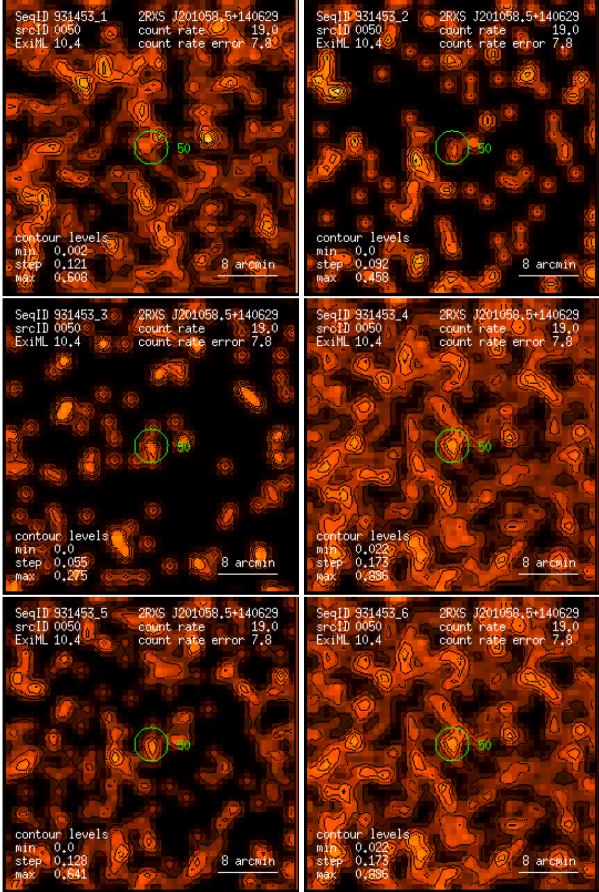
Figure 50: RASS 931453: detection 0050: band rate images, Gaussian filter: (1) PSPC channels 11 – 41, (2) 52 – 90, (3) 91 – 201, (4) 11 – 235, (5) 52 – 201, (6) 11 – 201. Broad band rates in counts/ks. Band rate contour levels in counts/ks/arcmin 2 .
