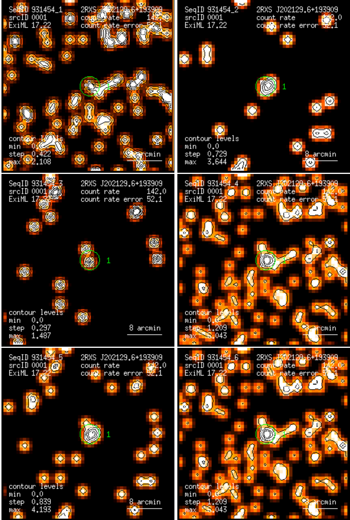
Figure 1: RASS 931454: detection 0001: band rate images, Gaussian filter: (1) PSPC channels 11 – 41, (2) 52 – 90, (3) 91 – 201, (4) 11 – 235, (5) 52 – 201, (6) 11 – 201. Broad band rates in counts/ks. Band rate contour levels in counts/ks/arcmin 2 .
