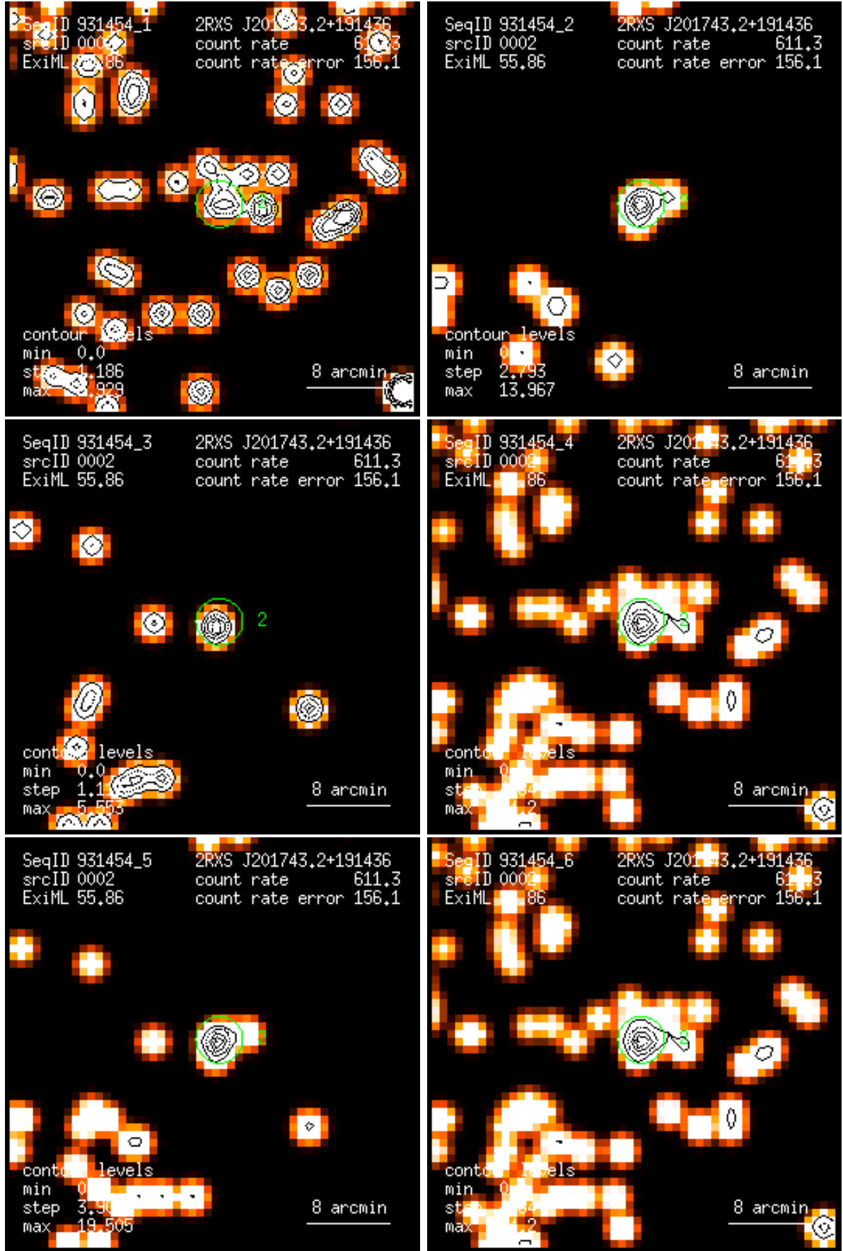
Figure 2: RASS 931454: detection 0002: band rate images, Gaussian filter: (1) PSPC channels 11 – 41, (2) 52 – 90, (3) 91 – 201, (4) 11 – 235, (5) 52 – 201, (6) 11 – 201. Broad band rates in counts/ks. Band rate contour levels in counts/ks/arcmin 2 .
