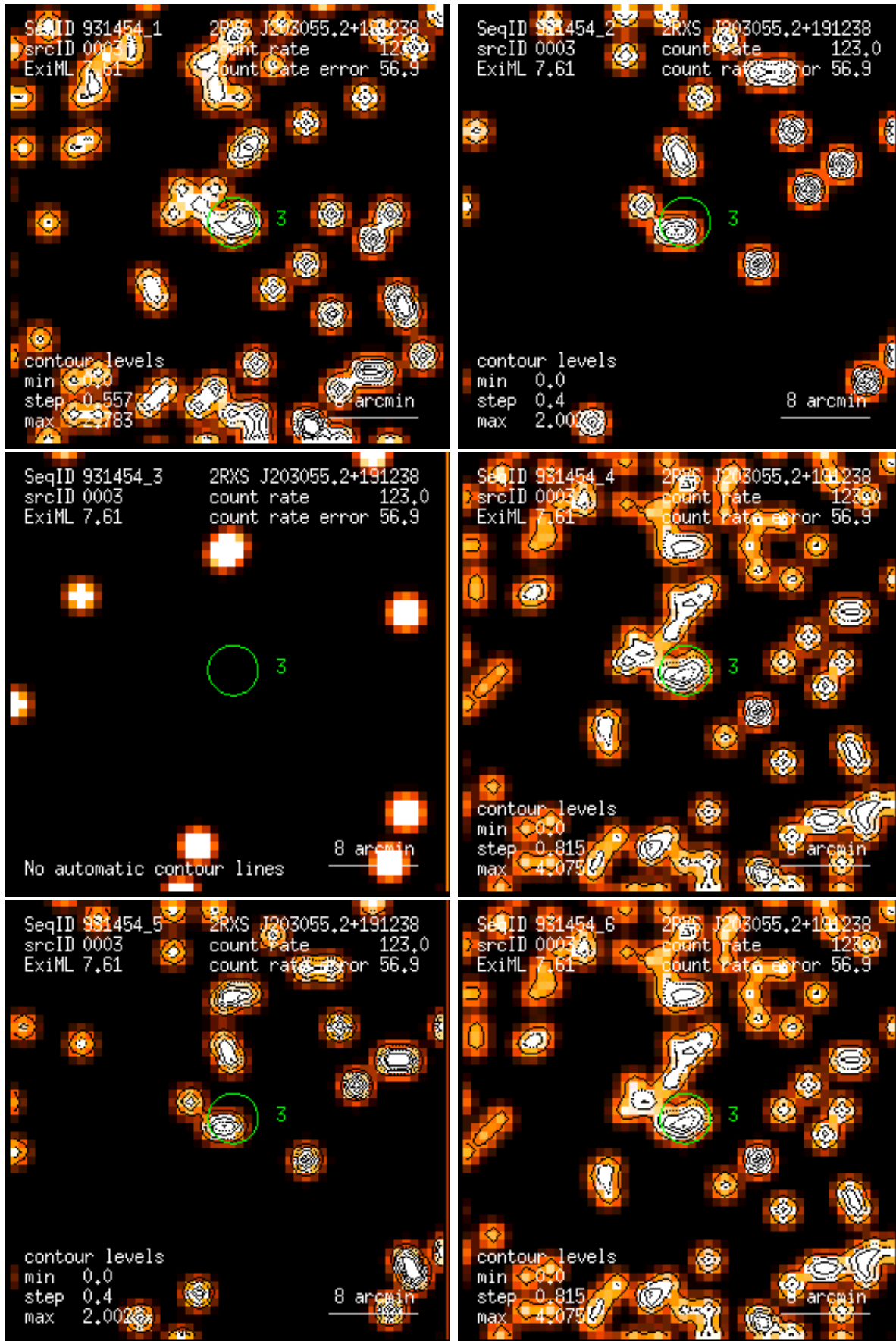
Figure 3: RASS 931454: detection 0003: band rate images, Gaussian filter: (1) PSPC channels 11 – 41, (2) 52 – 90, (3) 91 – 201, (4) 11 – 235, (5) 52 – 201, (6) 11 – 201. Broad band rates in counts/ks. Band rate contour levels in counts/ks/arcmin 2 .
