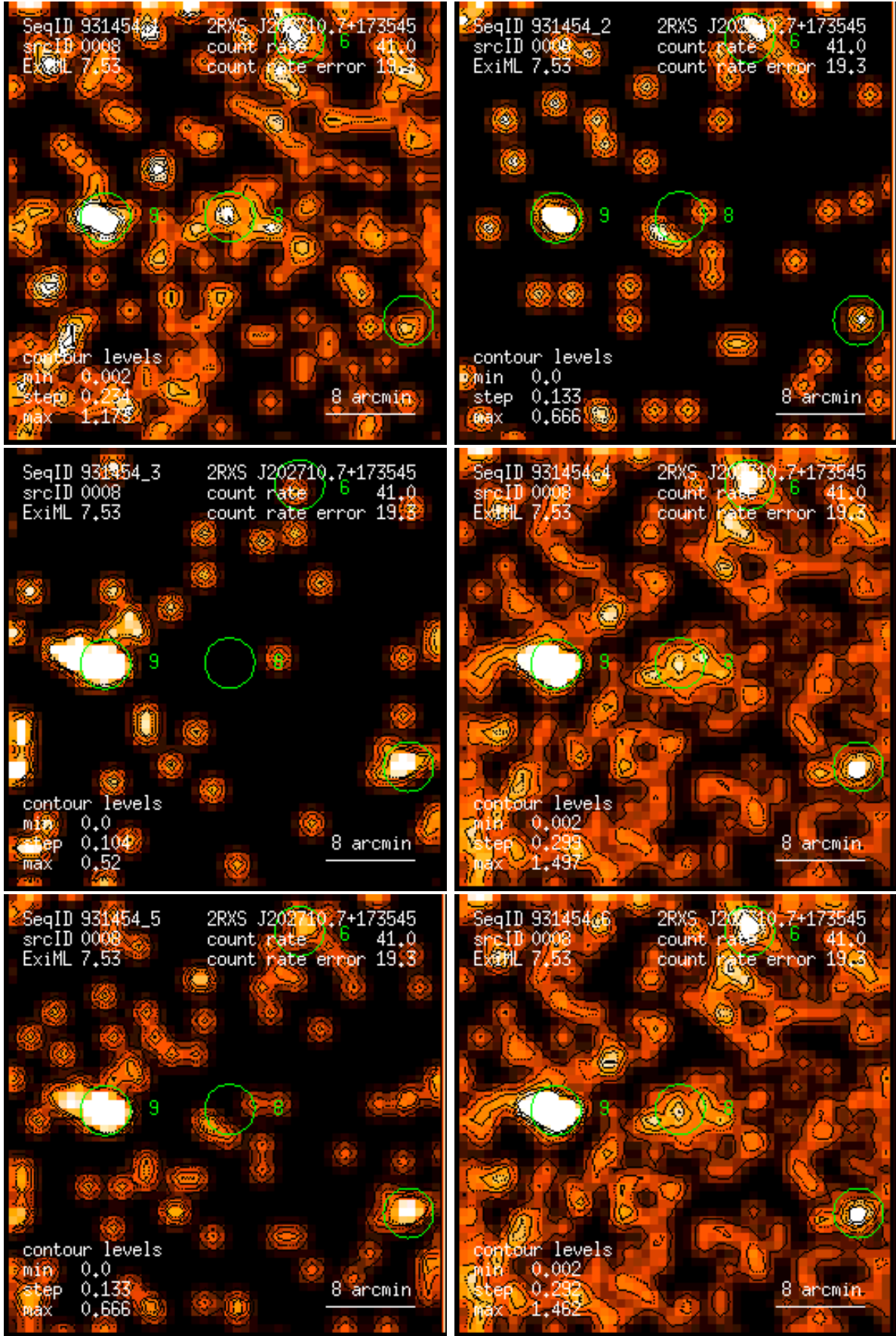
Figure 8: RASS 931454: detection 0008: band rate images, Gaussian filter: (1) PSPC channels 11 – 41, (2) 52 – 90, (3) 91 – 201, (4) 11 – 235, (5) 52 – 201, (6) 11 – 201. Broad band rates in counts/ks. Band rate contour levels in counts/ks/arcmin 2 .
