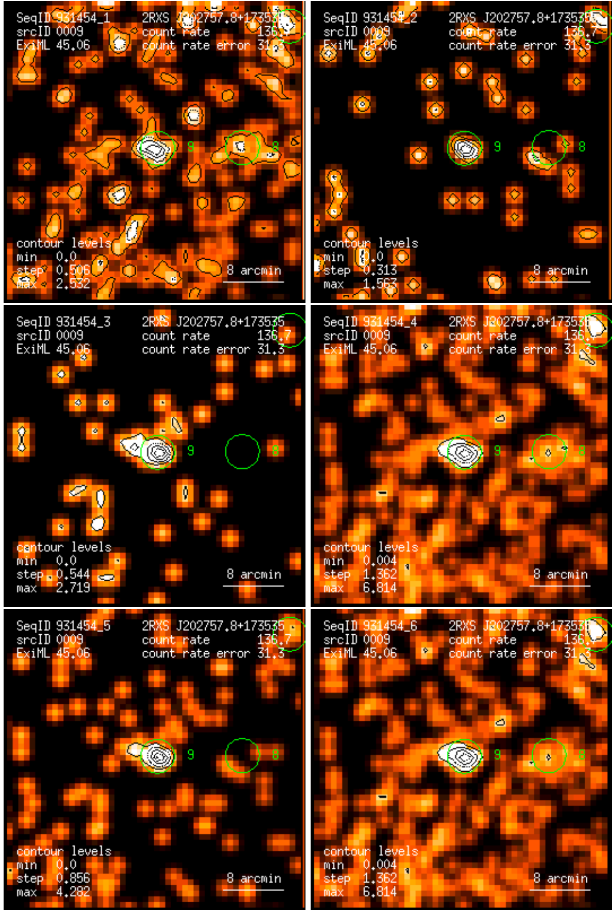
Figure 9: RASS 931454: detection 0009: band rate images, Gaussian filter: (1) PSPC channels 11 – 41, (2) 52 – 90, (3) 91 – 201, (4) 11 – 235, (5) 52 – 201, (6) 11 – 201. Broad band rates in counts/ks. Band rate contour levels in counts/ks/arcmin 2 .
