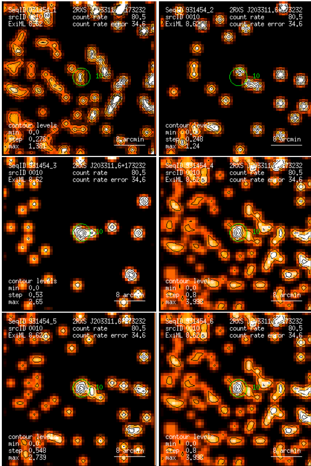
Figure 10: RASS 931454: detection 0010: band rate images, Gaussian filter: (1) PSPC channels 11 – 41, (2) 52 – 90, (3) 91 – 201, (4) 11 – 235, (5) 52 – 201, (6) 11 – 201. Broad band rates in counts/ks. Band rate contour levels in counts/ks/arcmin 2 .
