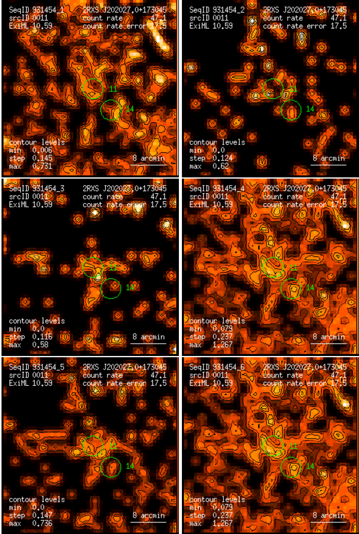
Figure 11: RASS 931454: detection 0011: band rate images, Gaussian filter: (1) PSPC channels 11 – 41, (2) 52 – 90, (3) 91 – 201, (4) 11 – 235, (5) 52 – 201, (6) 11 – 201. Broad band rates in counts/ks. Band rate contour levels in counts/ks/arcmin 2 .
