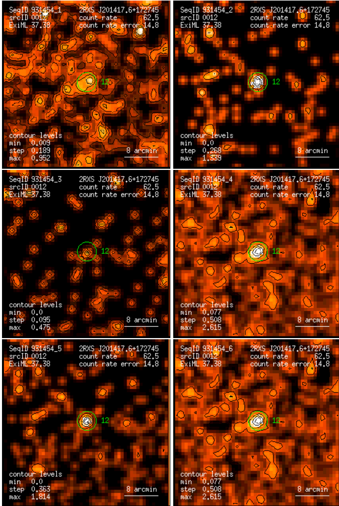
Figure 12: RASS 931454: detection 0012: band rate images, Gaussian filter: (1) PSPC channels 11 – 41, (2) 52 – 90, (3) 91 – 201, (4) 11 – 235, (5) 52 – 201, (6) 11 – 201. Broad band rates in counts/ks. Band rate contour levels in counts/ks/arcmin 2 .
