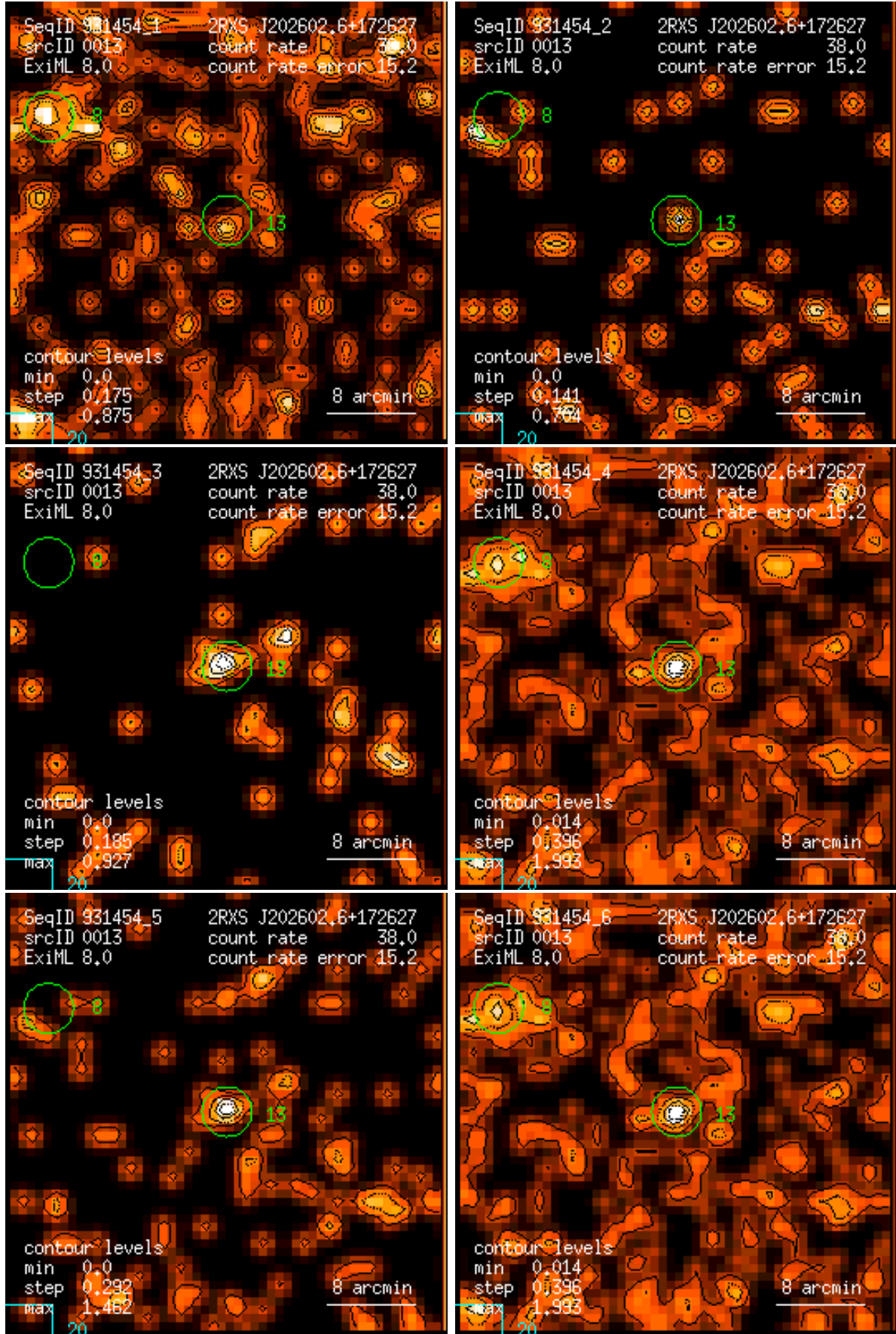
Figure 13: RASS 931454: detection 0013: band rate images, Gaussian filter: (1) PSPC channels 11 – 41, (2) 52 – 90, (3) 91 – 201, (4) 11 – 235, (5) 52 – 201, (6) 11 – 201. Broad band rates in counts/ks. Band rate contour levels in counts/ks/arcmin 2 .
