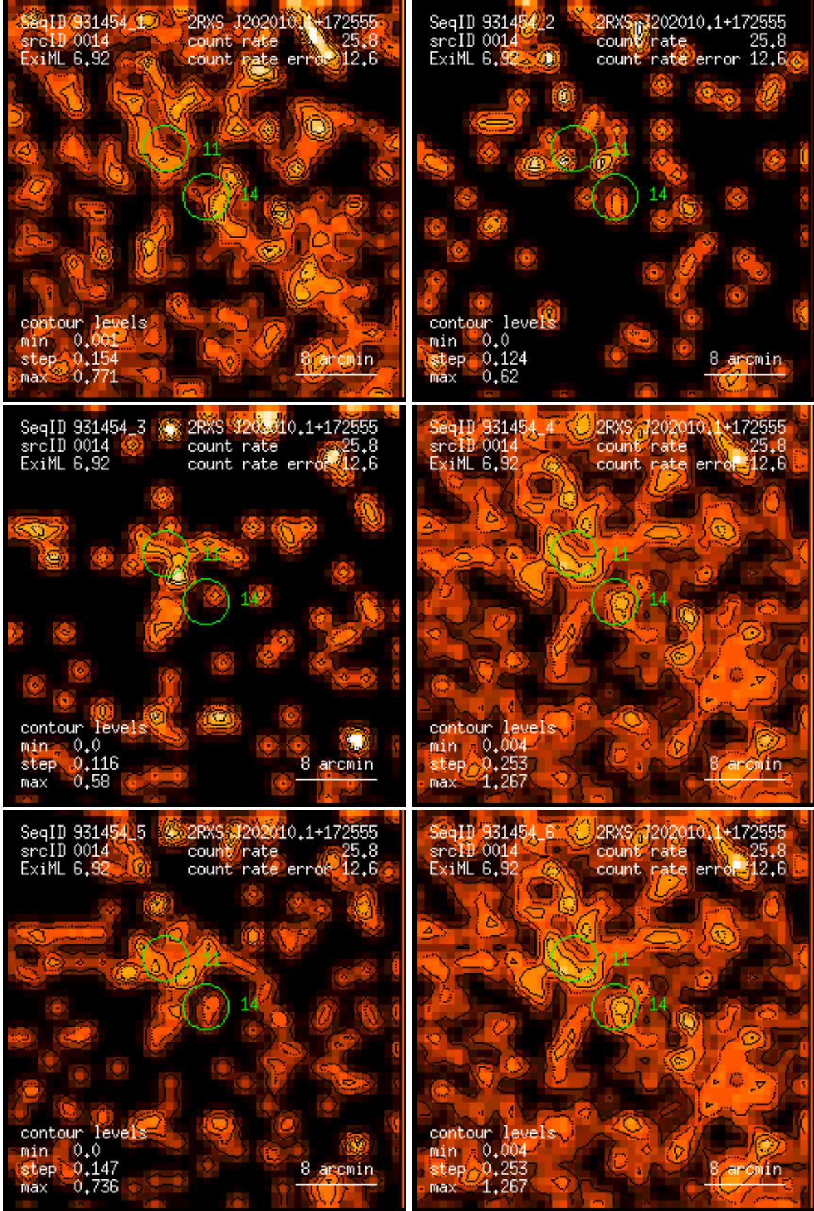
Figure 14: RASS 931454: detection 0014: band rate images, Gaussian filter: (1) PSPC channels 11 – 41, (2) 52 – 90, (3) 91 – 201, (4) 11 – 235, (5) 52 – 201, (6) 11 – 201. Broad band rates in counts/ks. Band rate contour levels in counts/ks/arcmin 2 .
