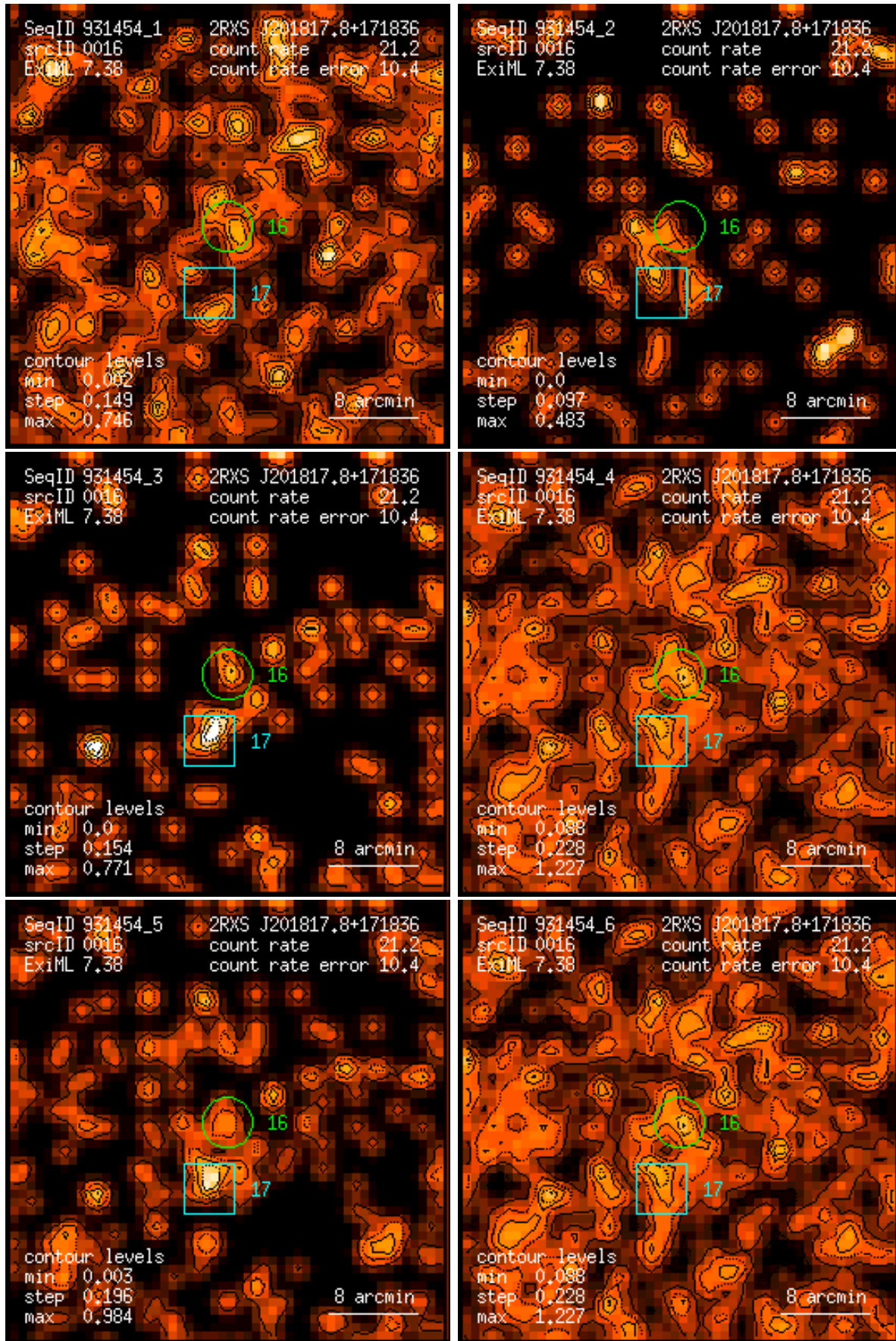
Figure 16: RASS 931454: detection 0016: band rate images, Gaussian filter: (1) PSPC channels 11 – 41, (2) 52 – 90, (3) 91 – 201, (4) 11 – 235, (5) 52 – 201, (6) 11 – 201. Broad band rates in counts/ks. Band rate contour levels in counts/ks/arcmin 2 .
