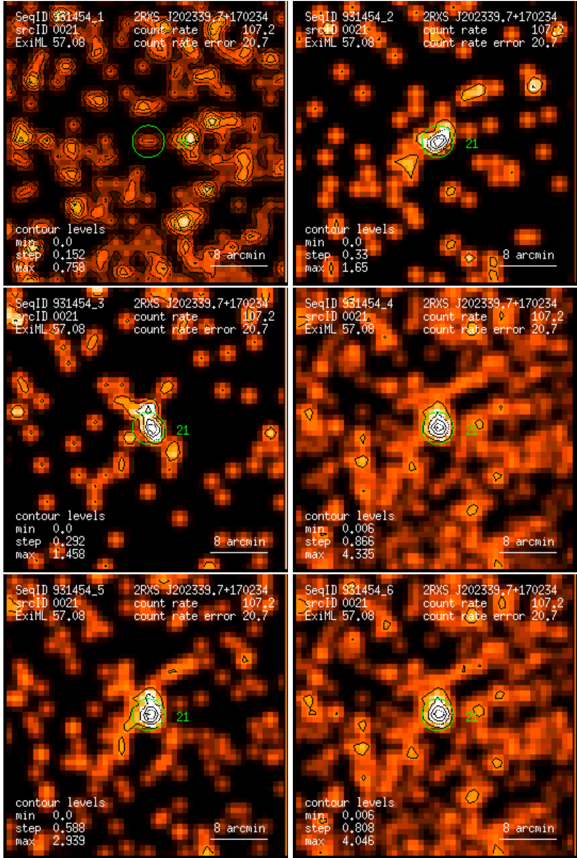
Figure 21: RASS 931454: detection 0021: band rate images, Gaussian filter: (1) PSPC channels 11 – 41, (2) 52 – 90, (3) 91 – 201, (4) 11 – 235, (5) 52 – 201, (6) 11 – 201. Broad band rates in counts/ks. Band rate contour levels in counts/ks/arcmin 2 .
